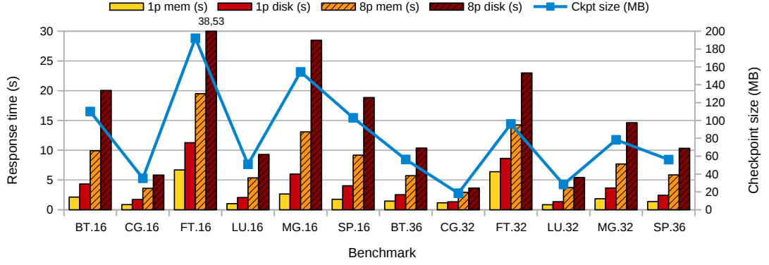
Figure 4.3: Response time (in seconds) in Pluton N1.
