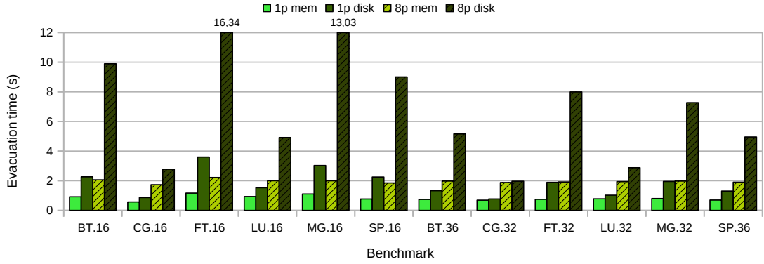
Figure 4.6: Evacuation time (in seconds) in Pluton N2.
