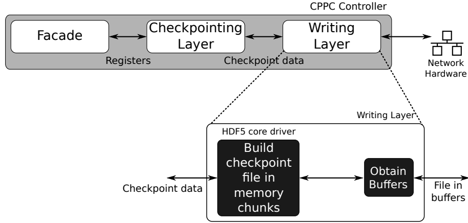
Figure 4.11: Modification of the CPPC writing layer
