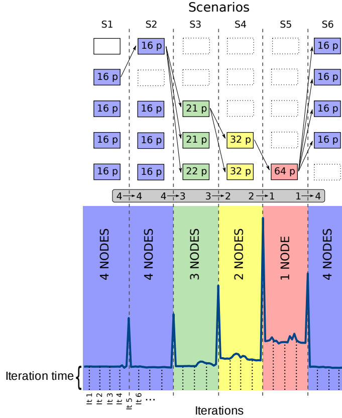
Figure 5.5: Testbed scenarios
