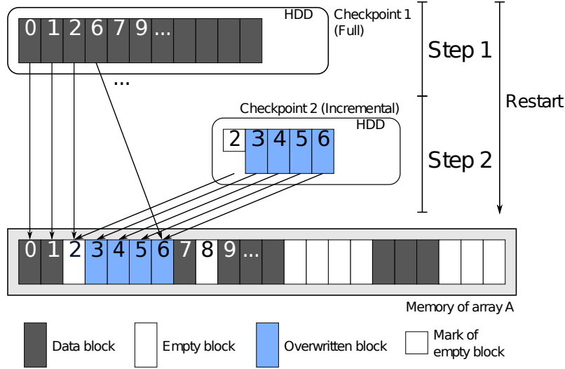
Figure 2.3: Restart from an incremental checkpoint.
