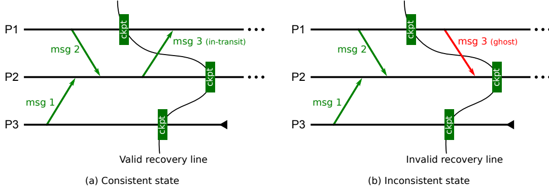
Figure 1.1: Example of valid and invalid recovery lines
